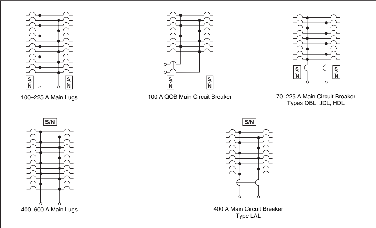
1-Phase, 3-Wire
